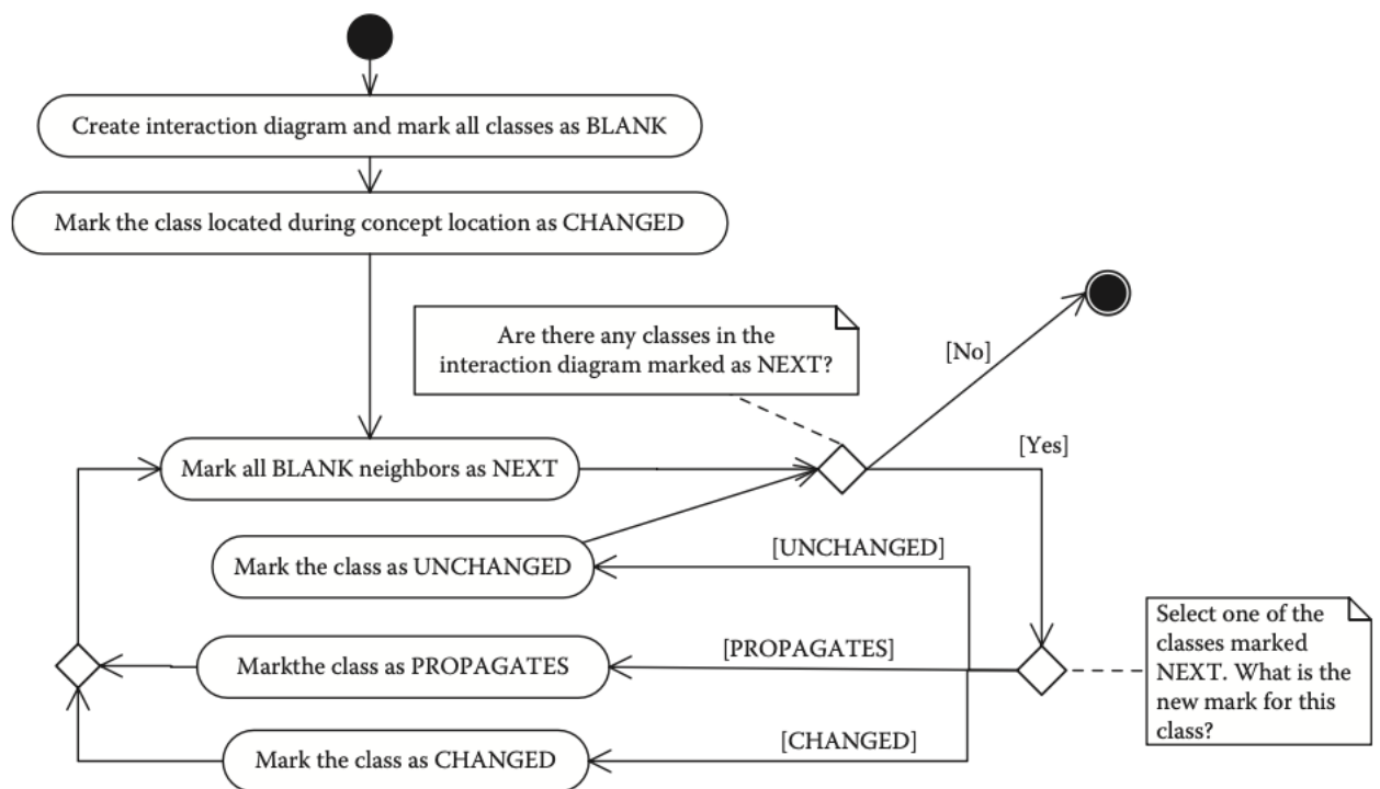
Figure 7.9 Activity diagram of impact analysis.
